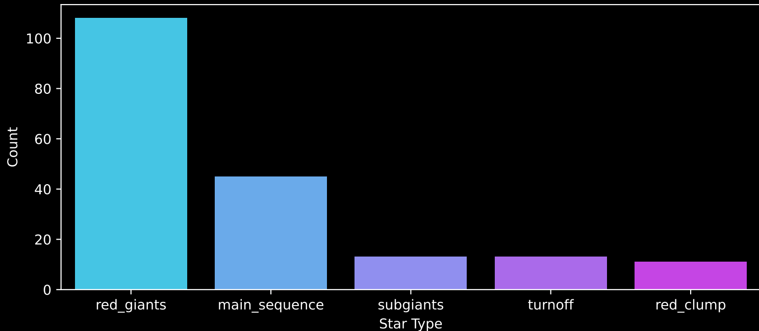
APOGEE DR17 Field: [188+18] Count plot of Star Type
