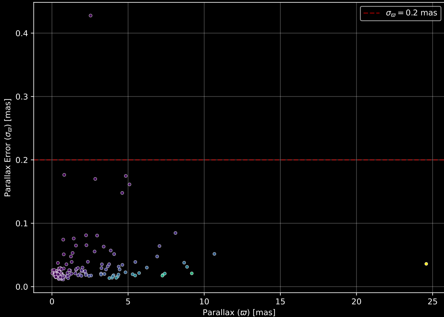
APOGEE DR17 Field: [188+18] Parallax Quality (n= 190)
