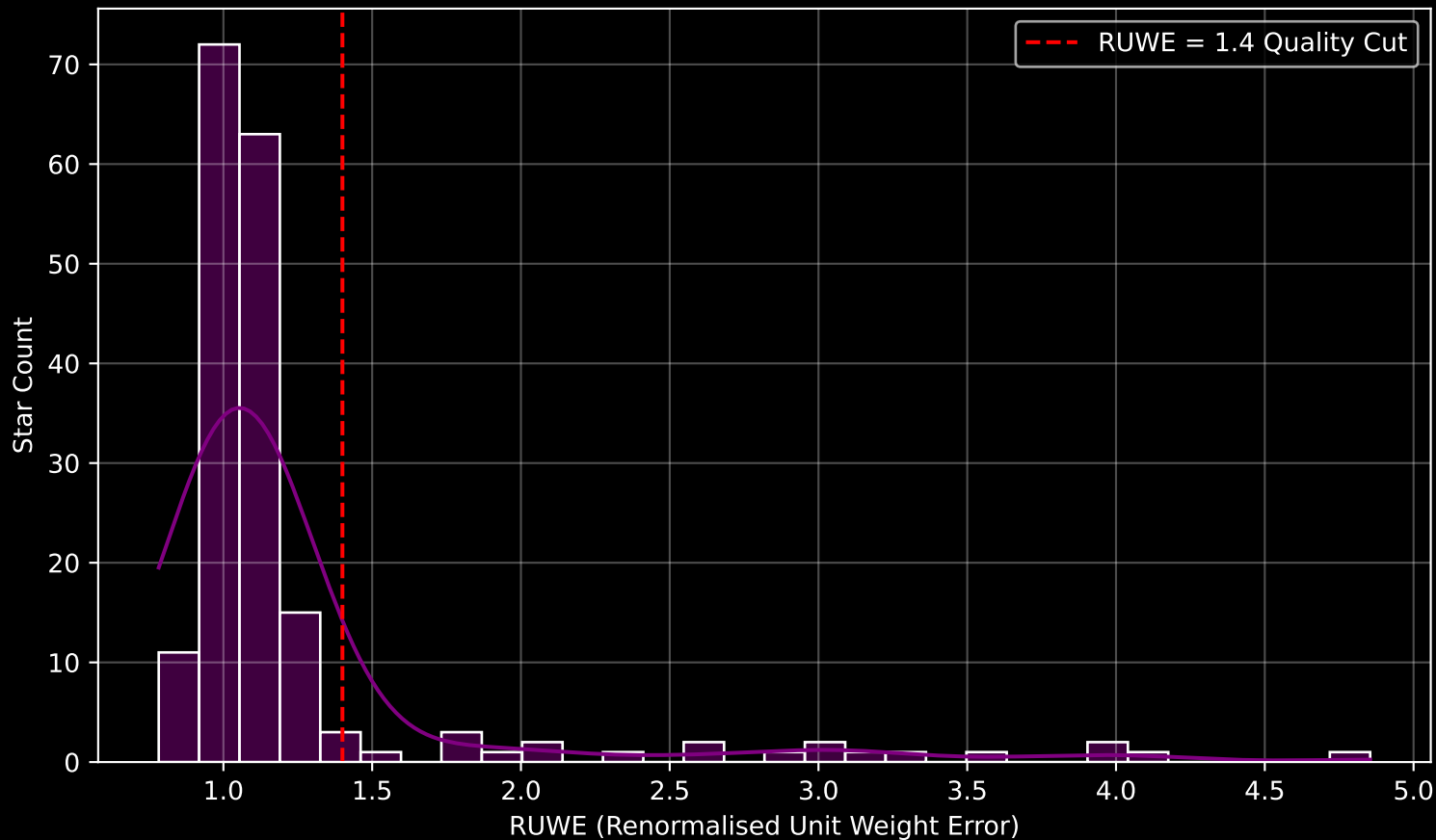
GAPOGEE DR17 Field [188+18] RUWE Distribution (n= 184)
