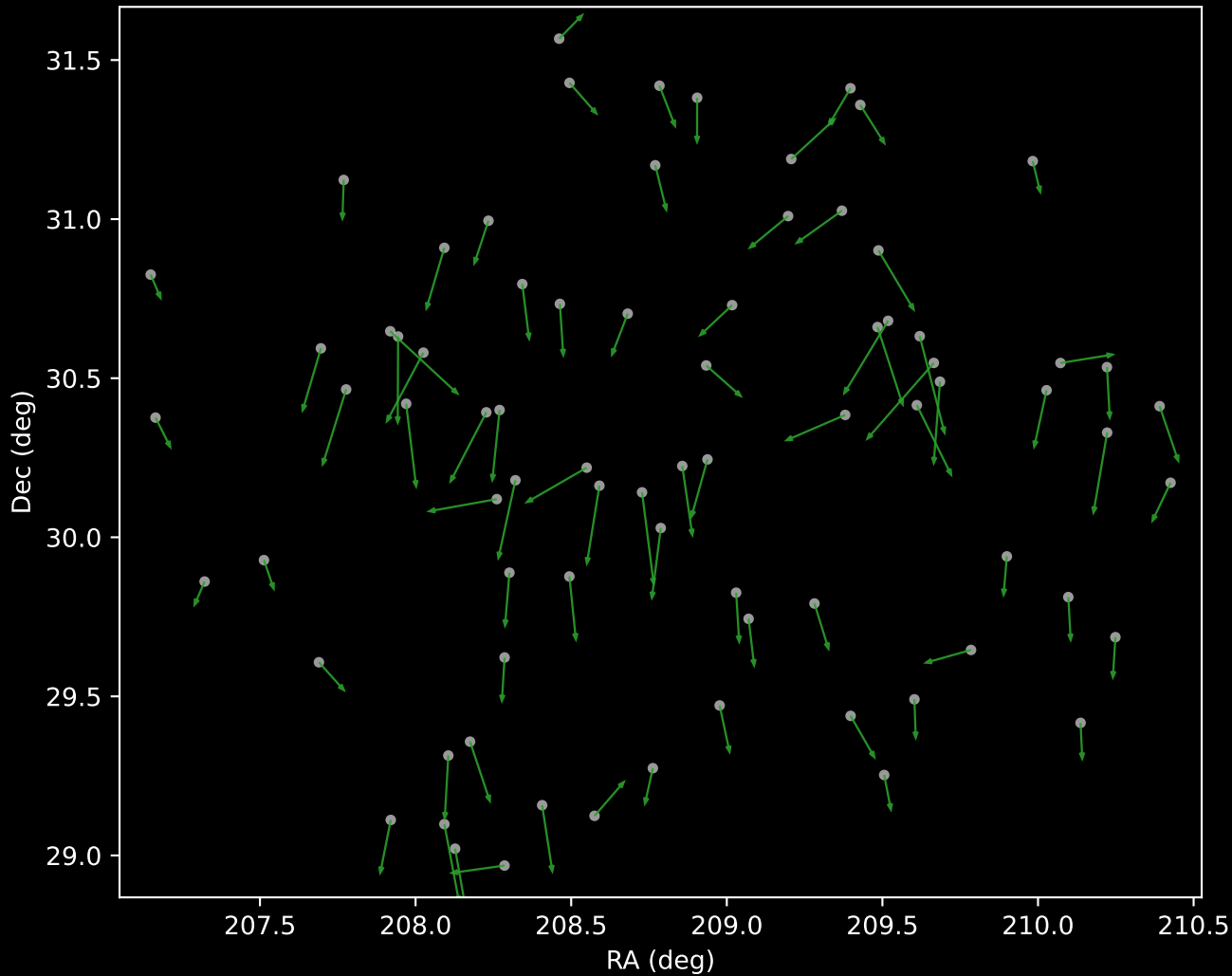
APOGEE DR17 Cluster 4 Proper Motion Vectors (n=78)
