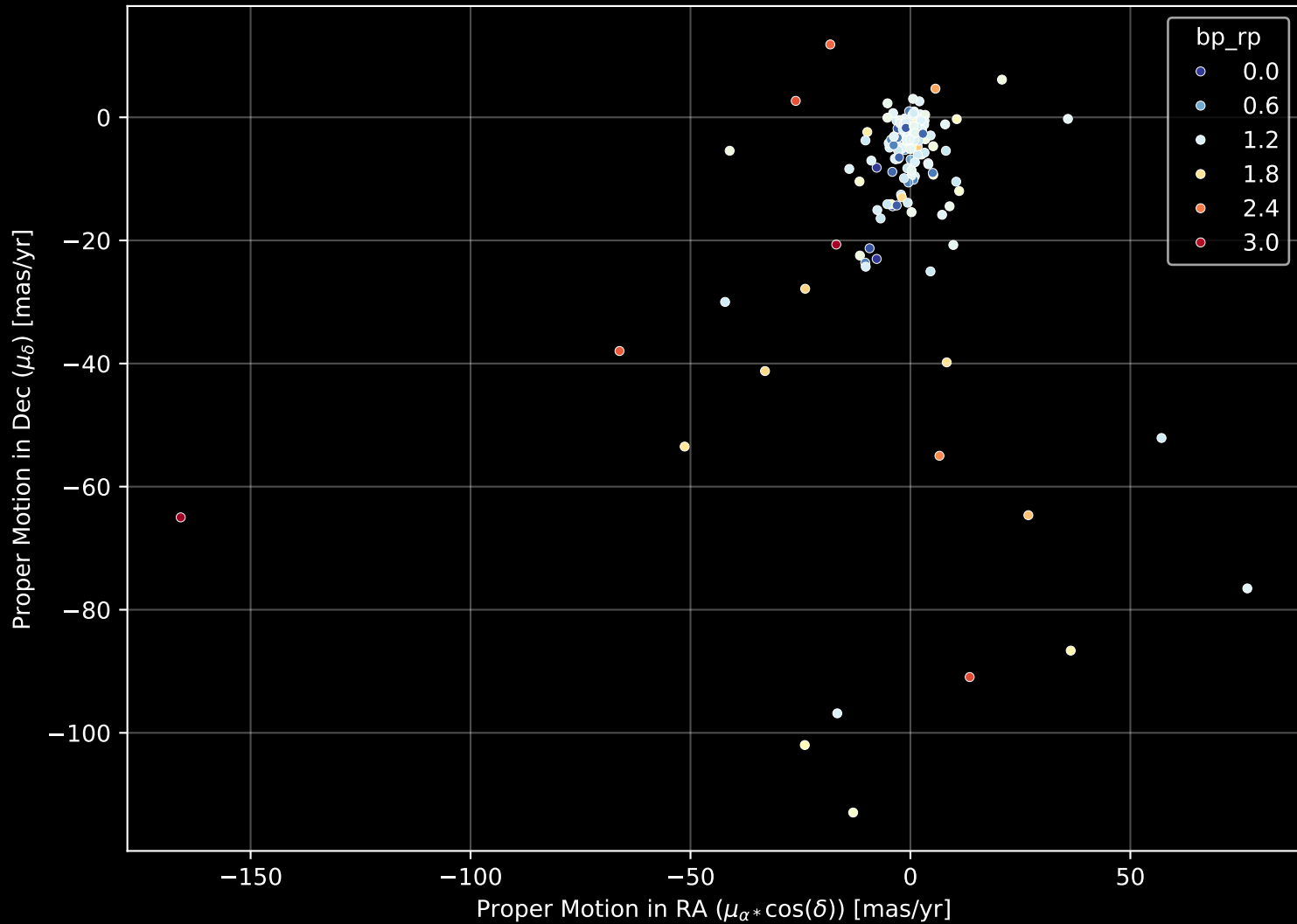
APOGEE DR17 Field: [188+18] Proper Motion Diagram (n= 190)
