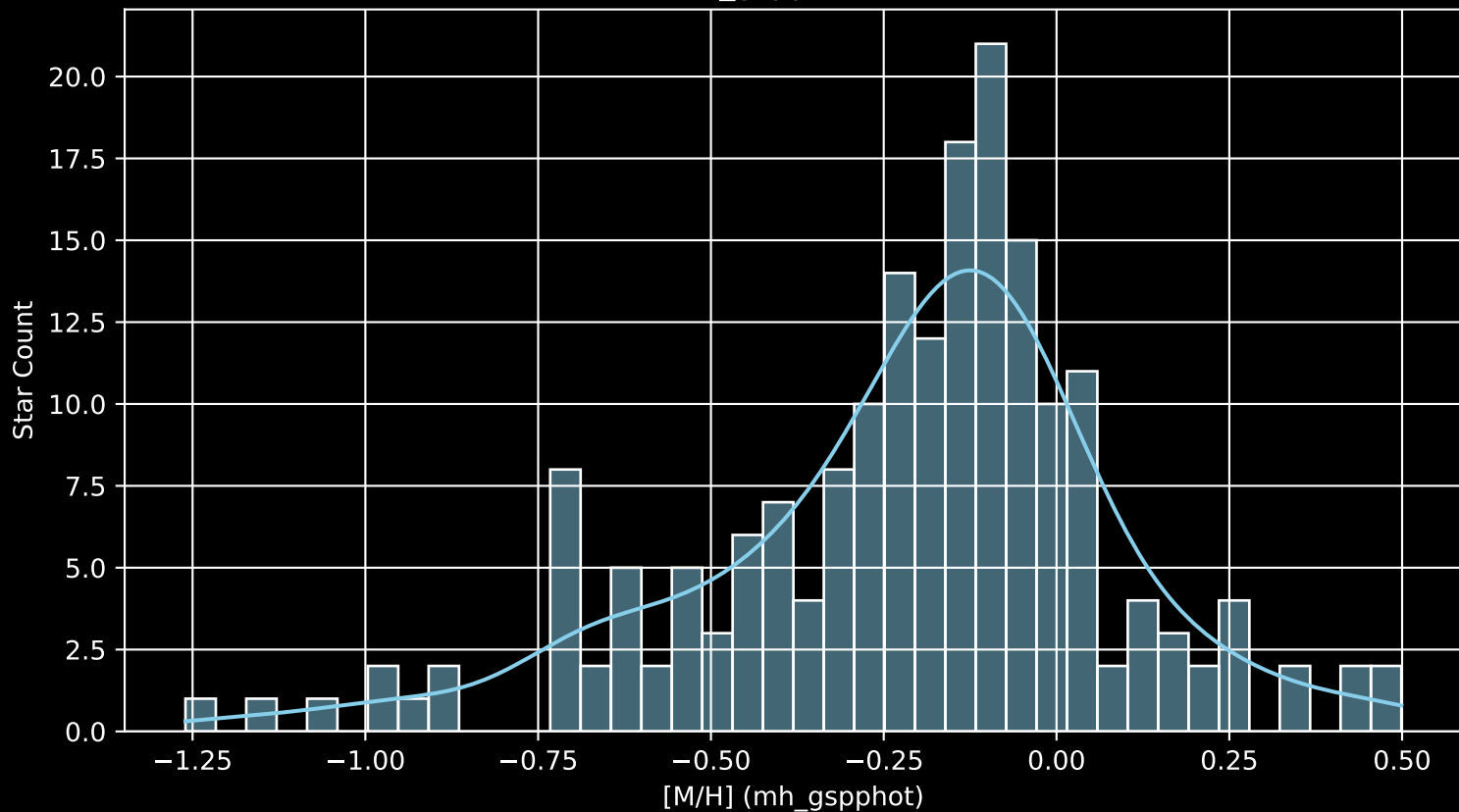
APOGEE DR17 Field: [188+18 [M/H] (mh_gspphot) (n= 190)
